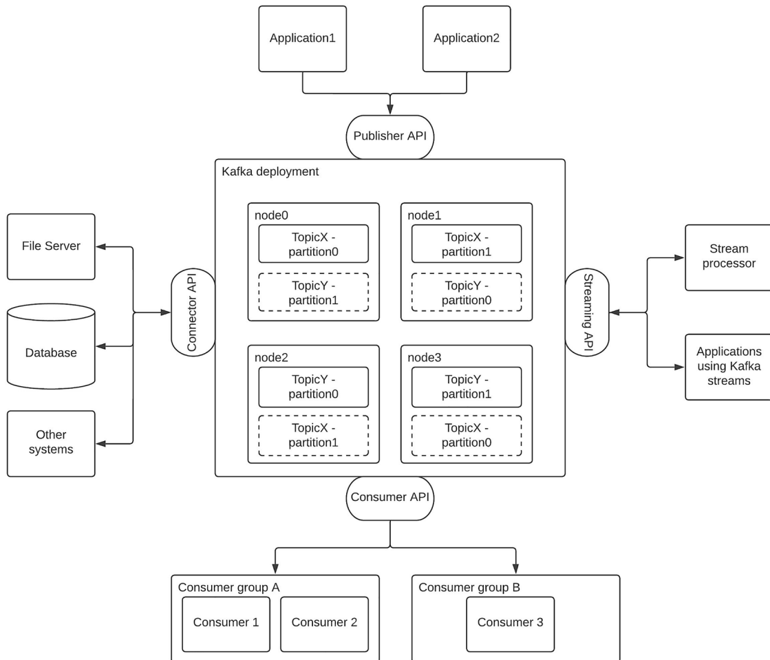
Figure 5-8 Kafka architecture in a nutshell
