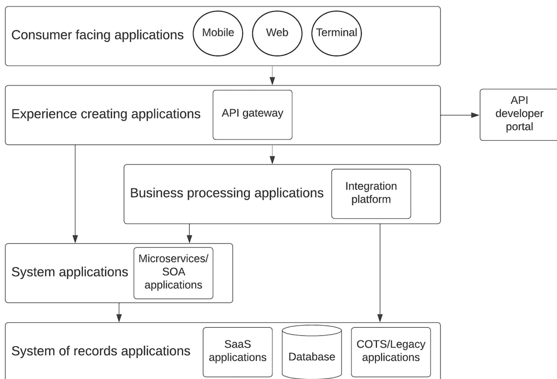
Figure 4-9 Layered architecture with real-world software components
