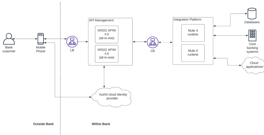
Figure 2-5 Deployment architecture for a mobile banking application
