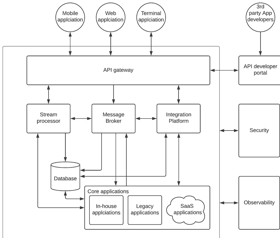
Figure 5-7 Event-driven enterprise software reference architecture
