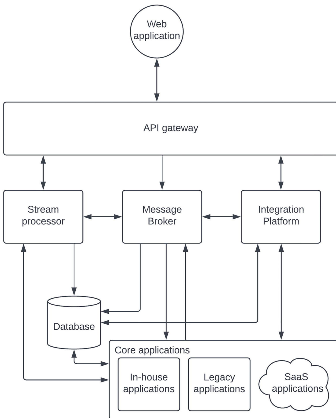
Figure 5-6 Event-driven enterprise-based architecture
