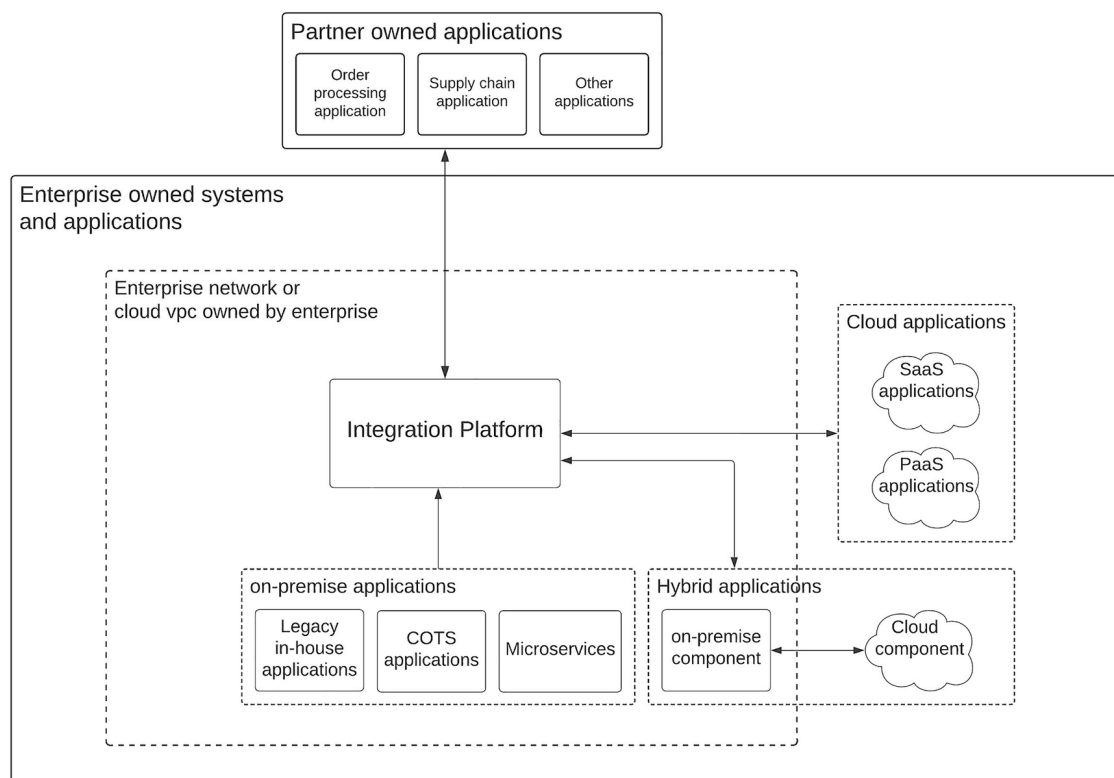
Figure 4-4 Business integration with integration platform
