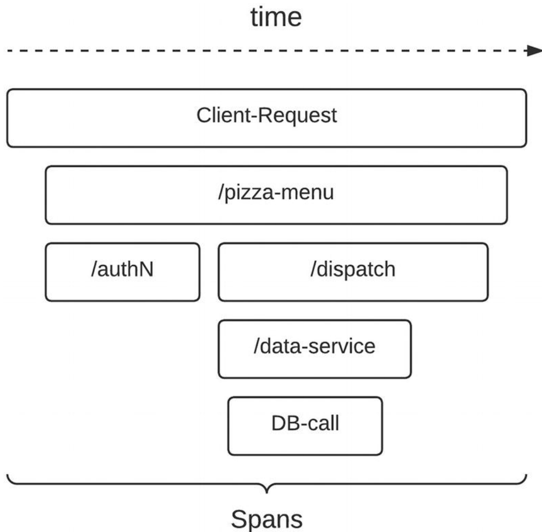
Figure 7-5 Spans in a distributed tracing scenario
