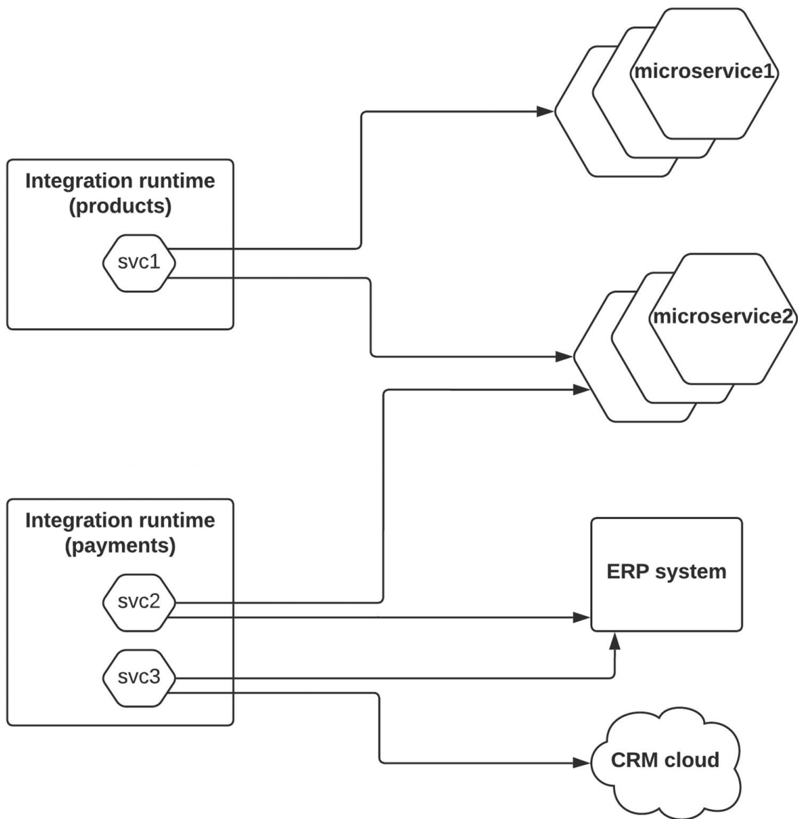
Figure 3-4 Creating integration microservices
