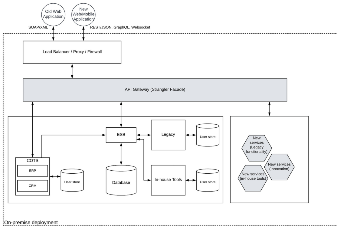
Figure 4-13 Legacy platform modernization with a strangler facade
