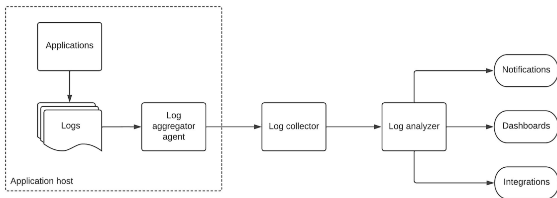
Figure 7-2 Observability with logs
