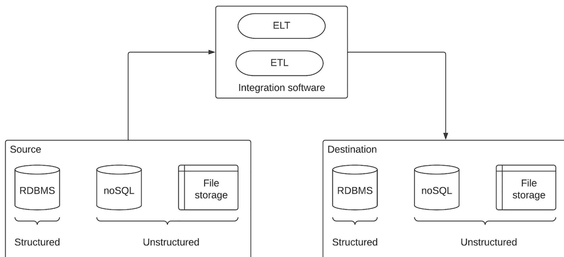
Figure 4-2 Data integration with ETL and ELT tasks
