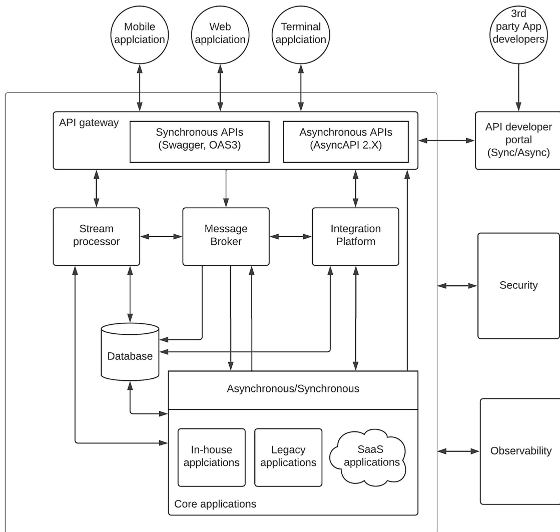
Figure 5-14 Event-driven enterprise architecture with sync/async APIs
