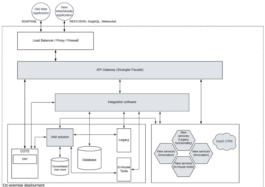
Figure 4-15 Legacy platform modernization with API, Integration and IAM solution
