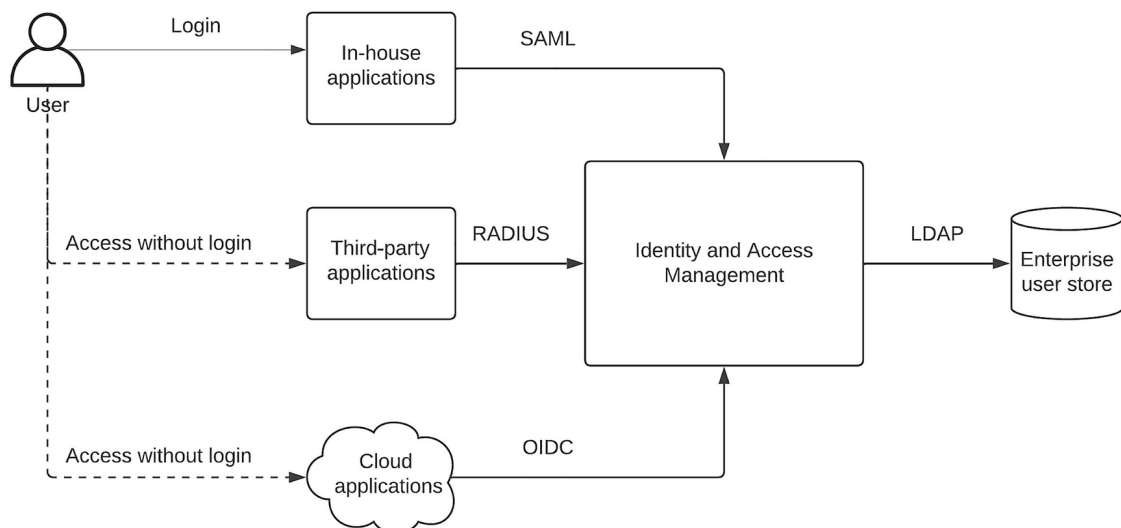
Figure 6-4 Single Sign-On with heterogeneous protocols
