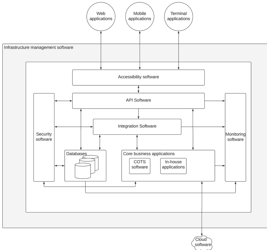
Figure 3-1 Key software components of an enterprise software system
