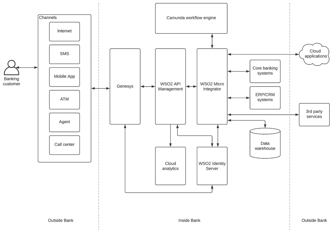
Figure 2-8 Technical architecture for an omni-channel banking solution
