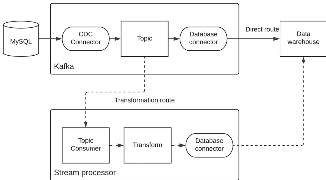
Figure 5-11 CDC pattern with Kafka
