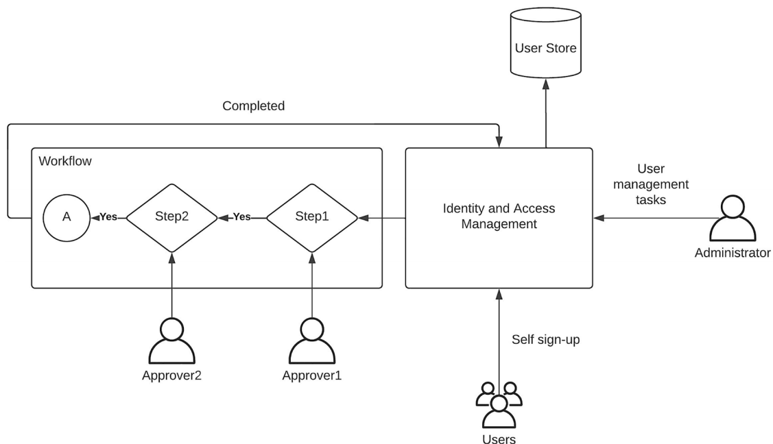
Figure 6-9 User management with approvals
