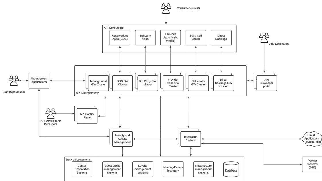
Figure 9-11 Solution architecture for a scalable hospitality platform
