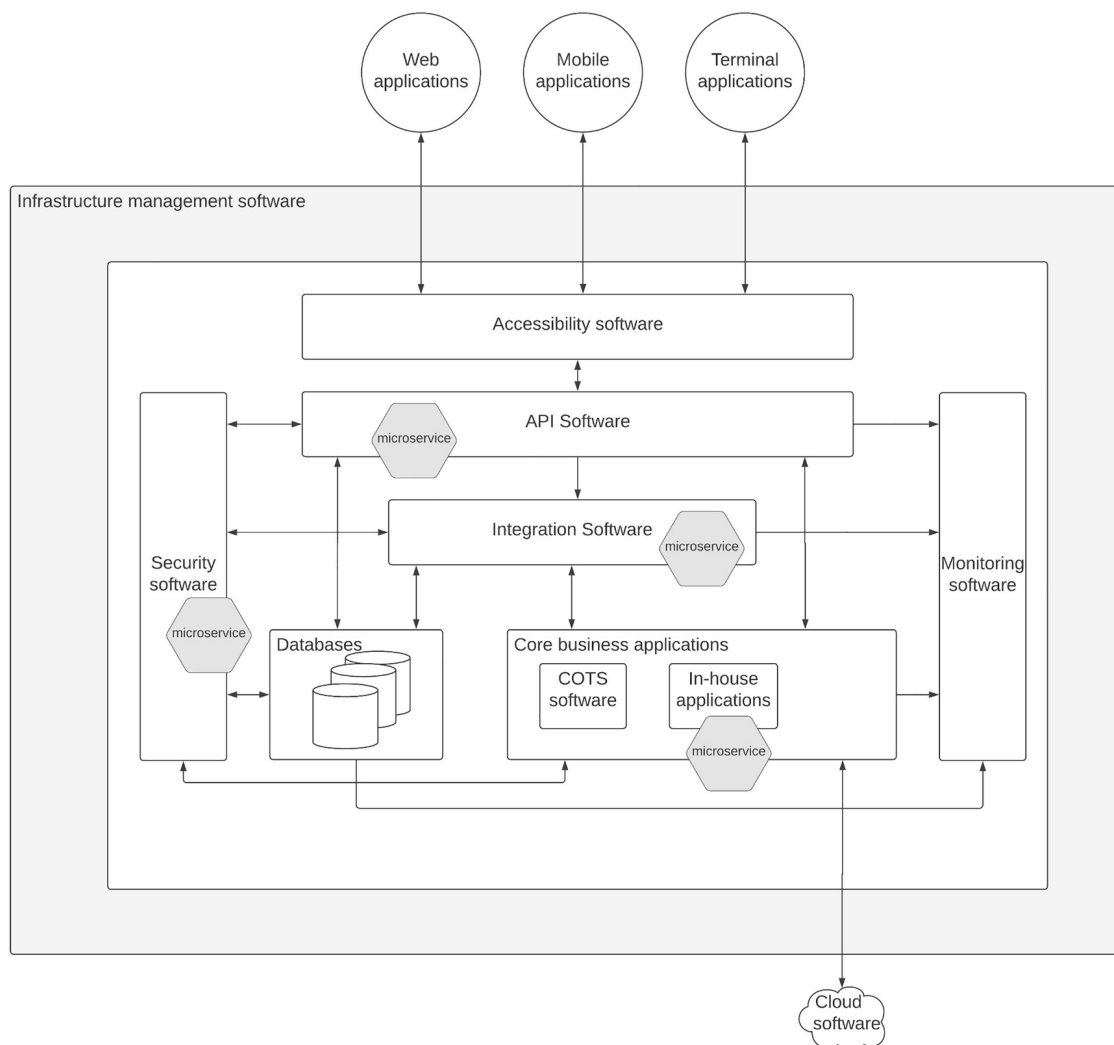
Figure 3-2 Microservice architecture-compatible components of an enterprise software system
