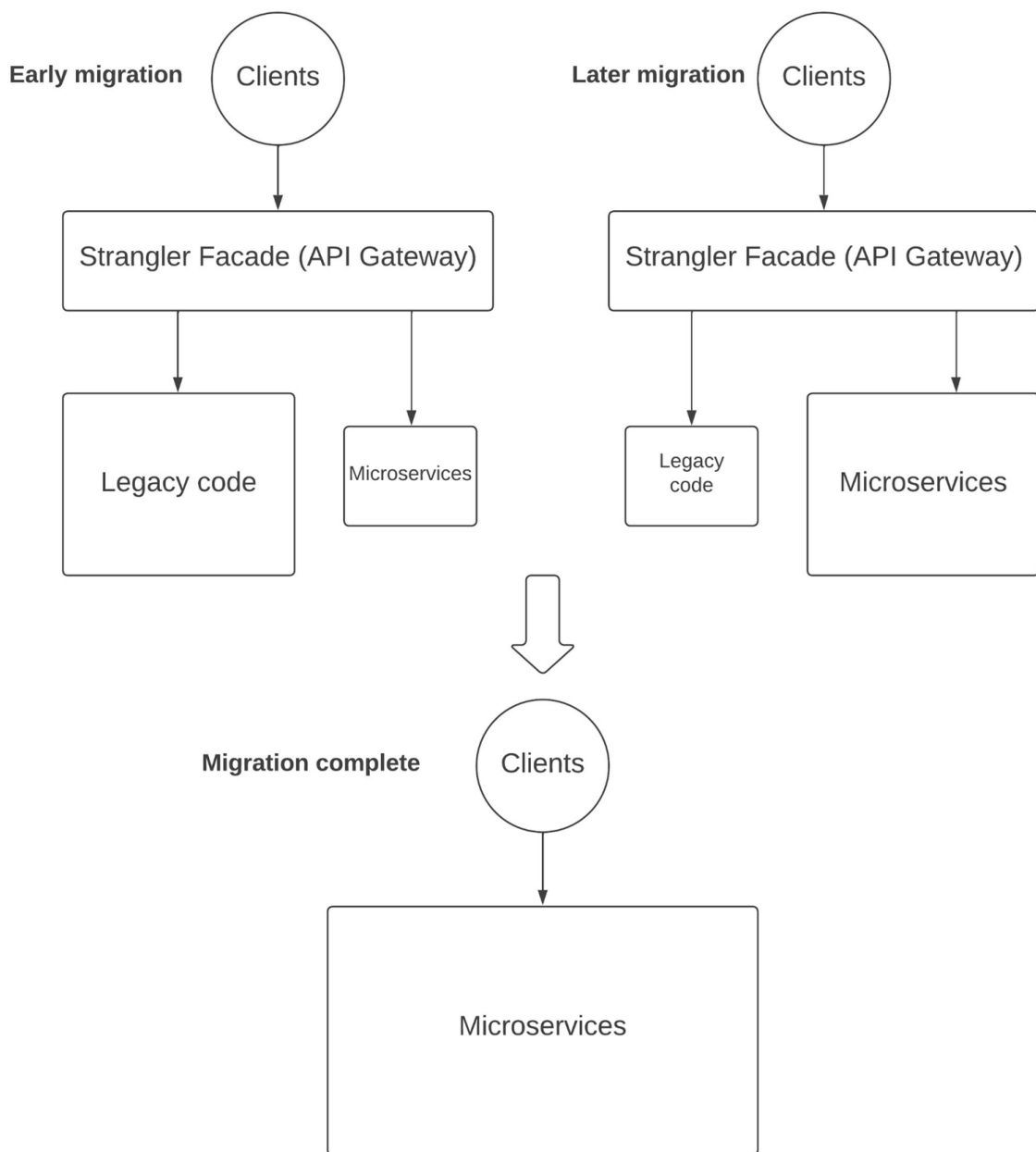
Figure 3-3 Migrating to microservice architecture with strangler pattern
