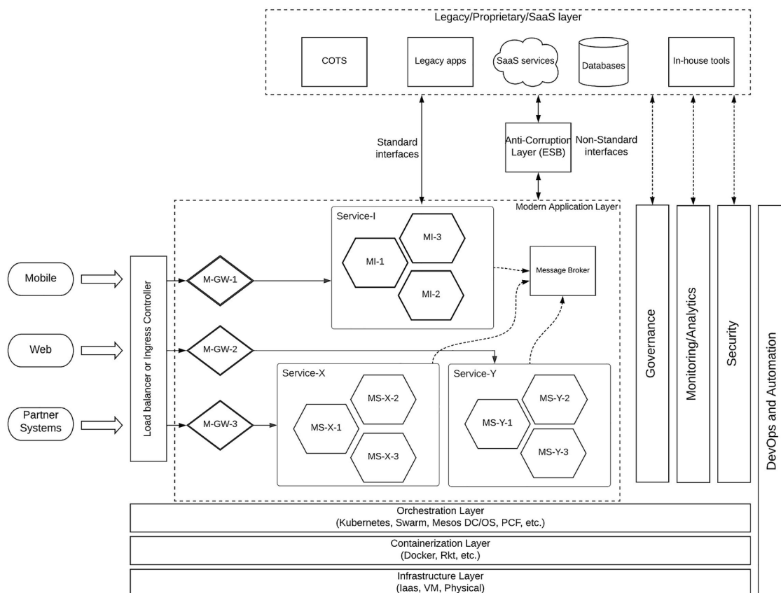
Figure 2-2 Microservices-based enterprise architecture pattern
