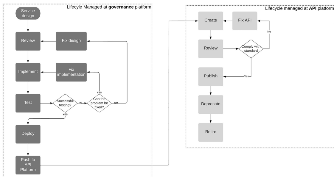
Figure 3-16 Integrating life cycle management of microservices with APIs
