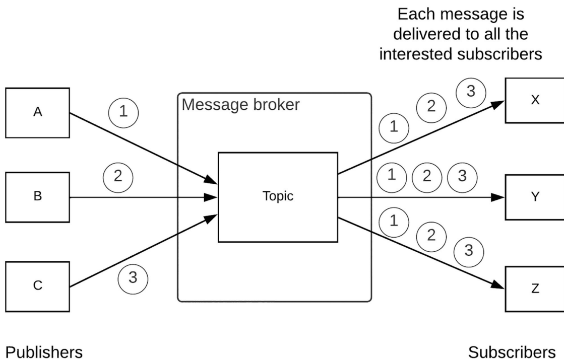
Figure 5-1 Topic-based publish-subscribe pattern
