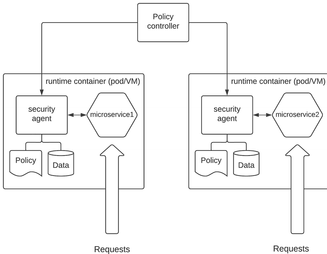
Figure 3-7 Decentralized security for microservices
