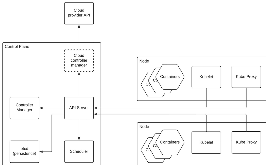
Figure 8-6 Kubernetes architecture
