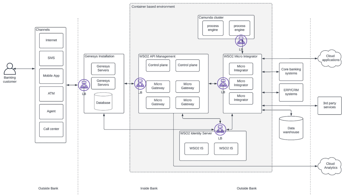
Figure 2-9 Deployment architecture for an omni-channel banking solution
