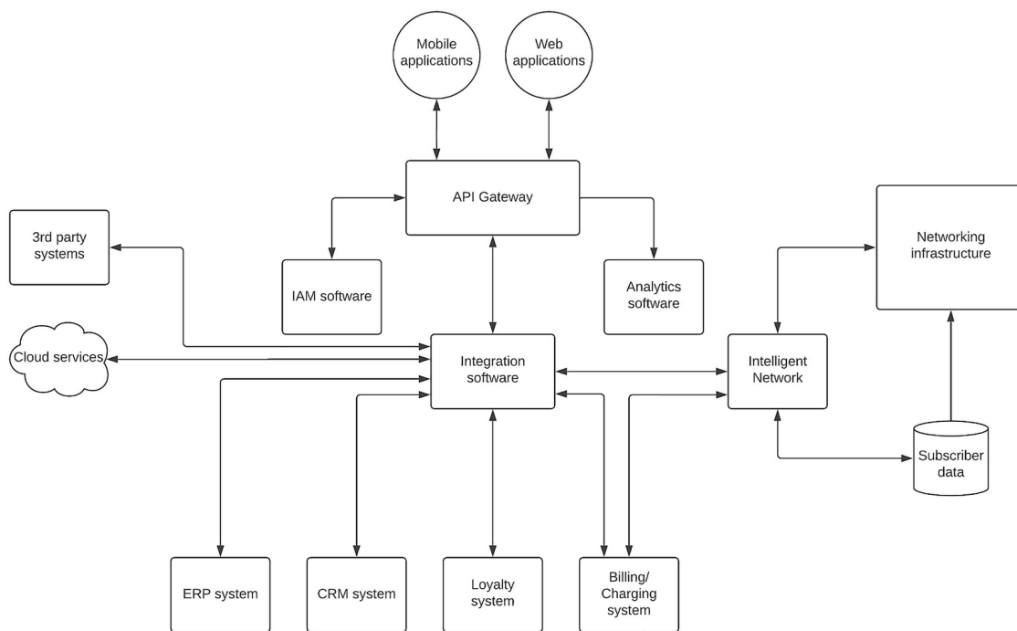
Figure 9-2 Solution architecture for a telecommunication IT system
