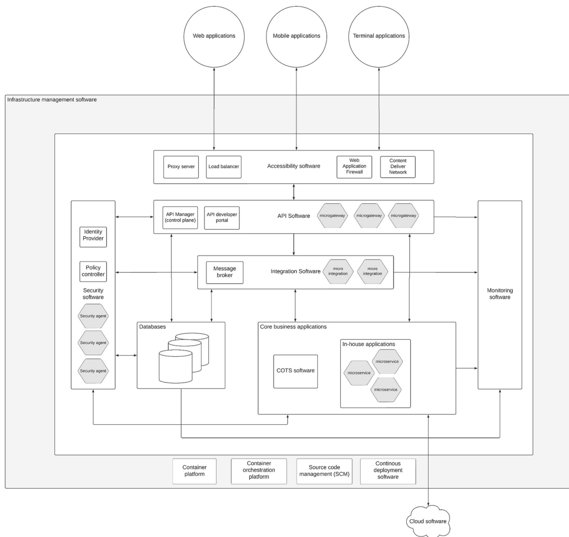
Figure 3-8 Enterprise software system reference architecture with MSA
