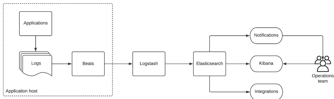
Figure 7-3 Log-based observability with ELK
