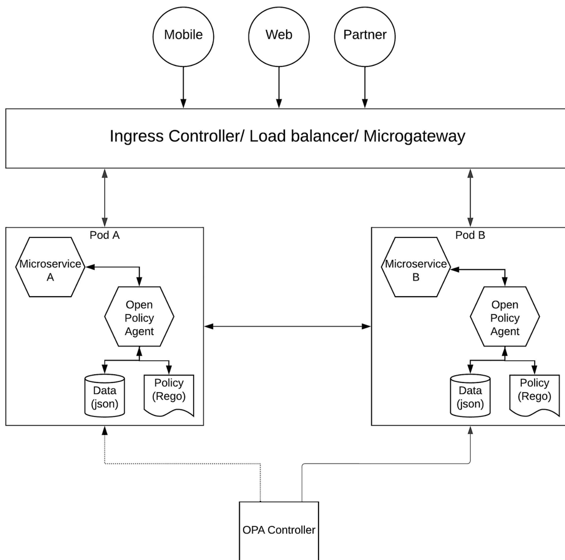
Figure 3-13 Microservice security with open policy agent
