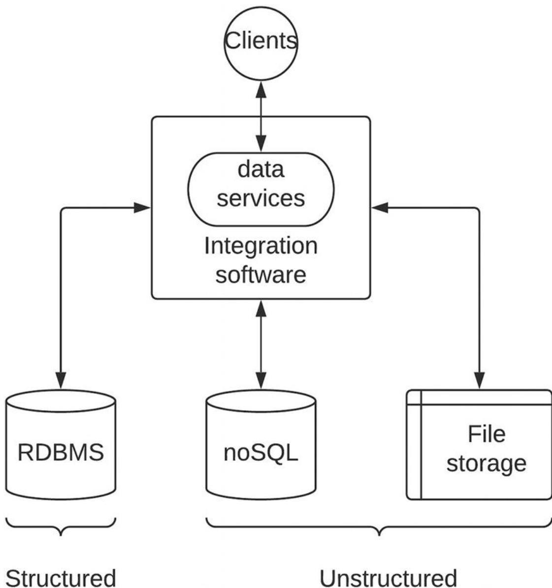
Figure 4-1 Integrating different data sources and exposing as data services
