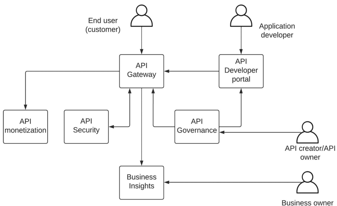
Figure 4-6 API platform components
