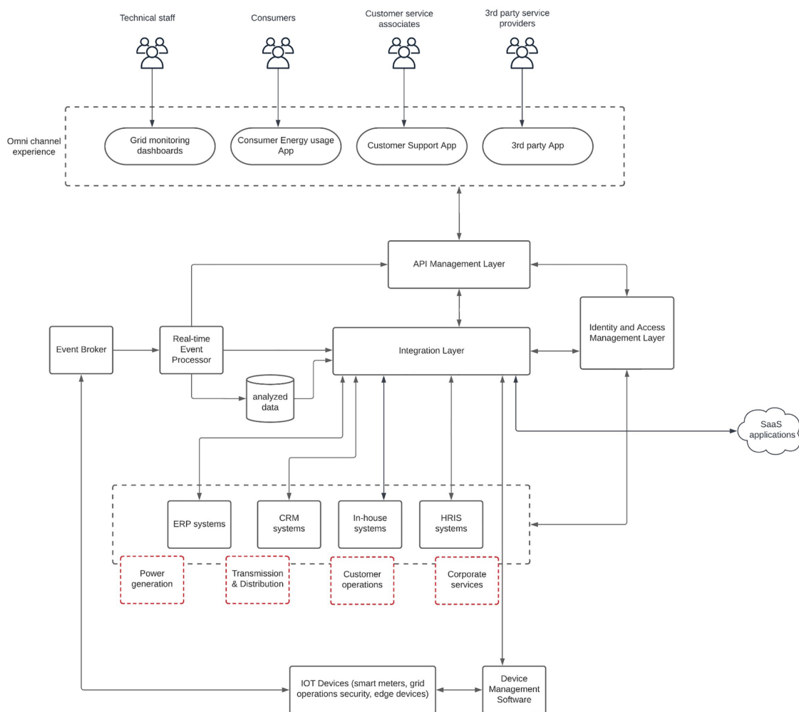
Figure 9-10 Solution architecture for energy industry
