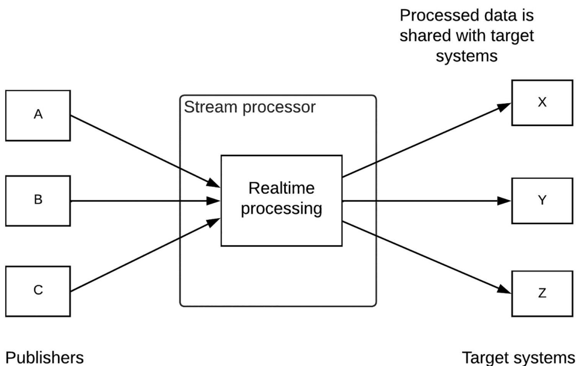
Figure 5-4 Real-time stream processing pattern
