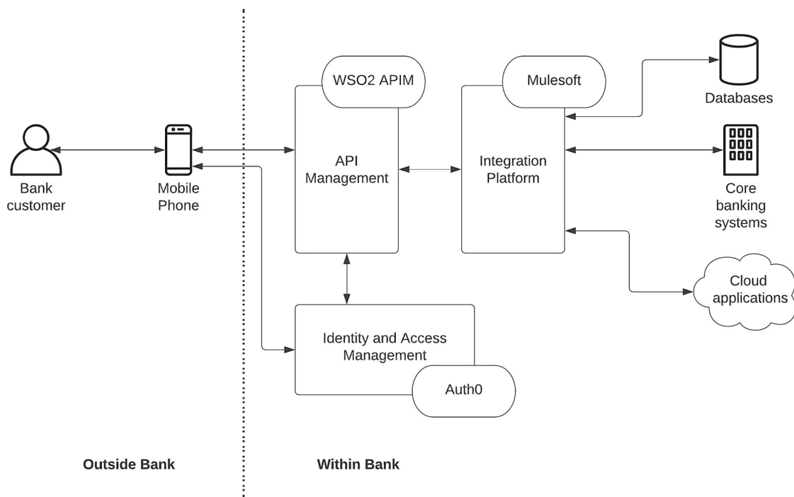
Figure 2-4 Technical solution architecture for a mobile banking application
