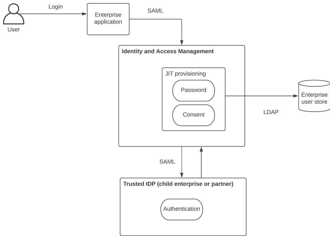
Figure 6-7 JIT provisioning for enterprise security
