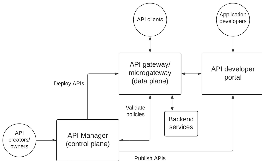
Figure 3-5 API management components
