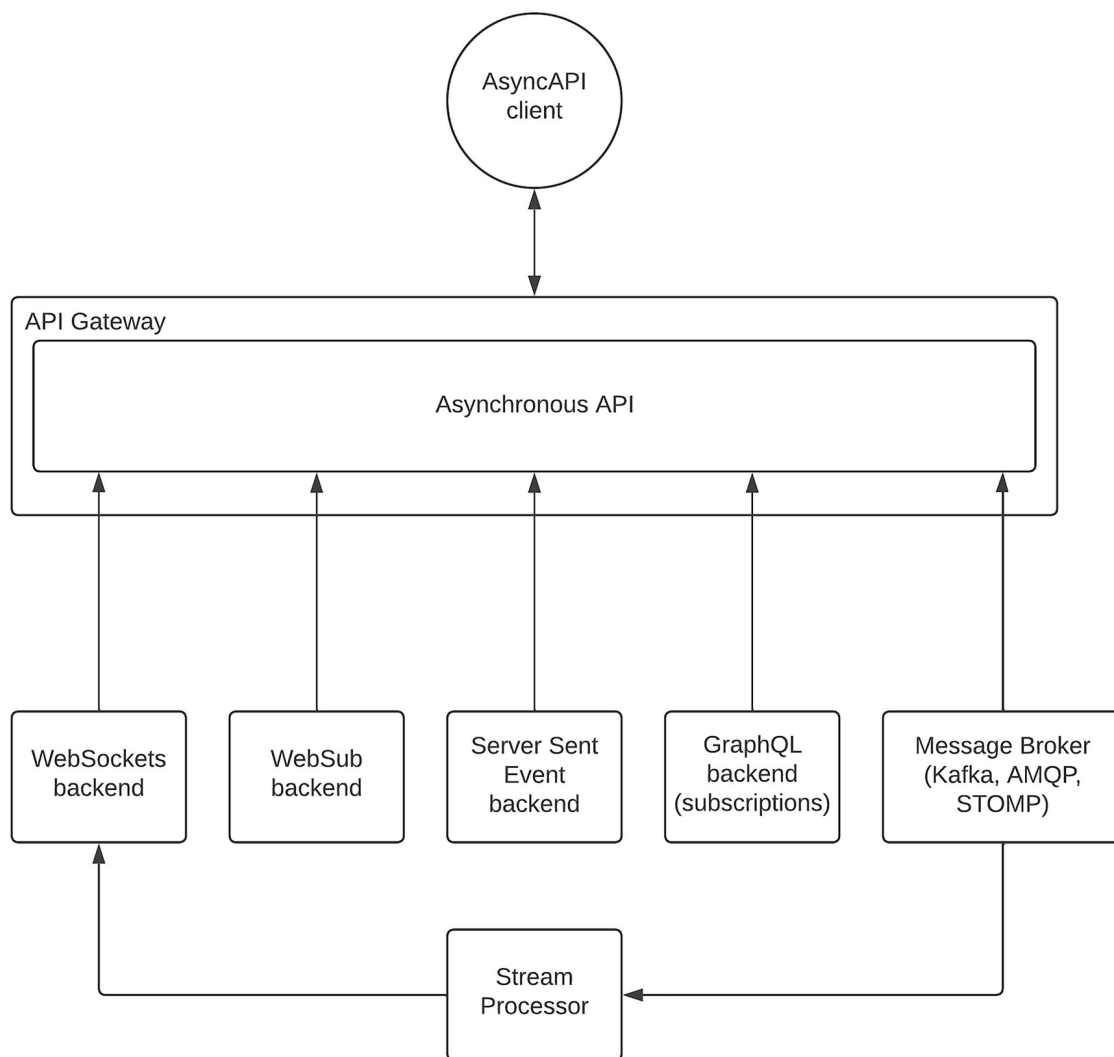
Figure 5-13 Asynchronous APIs with API gateway
