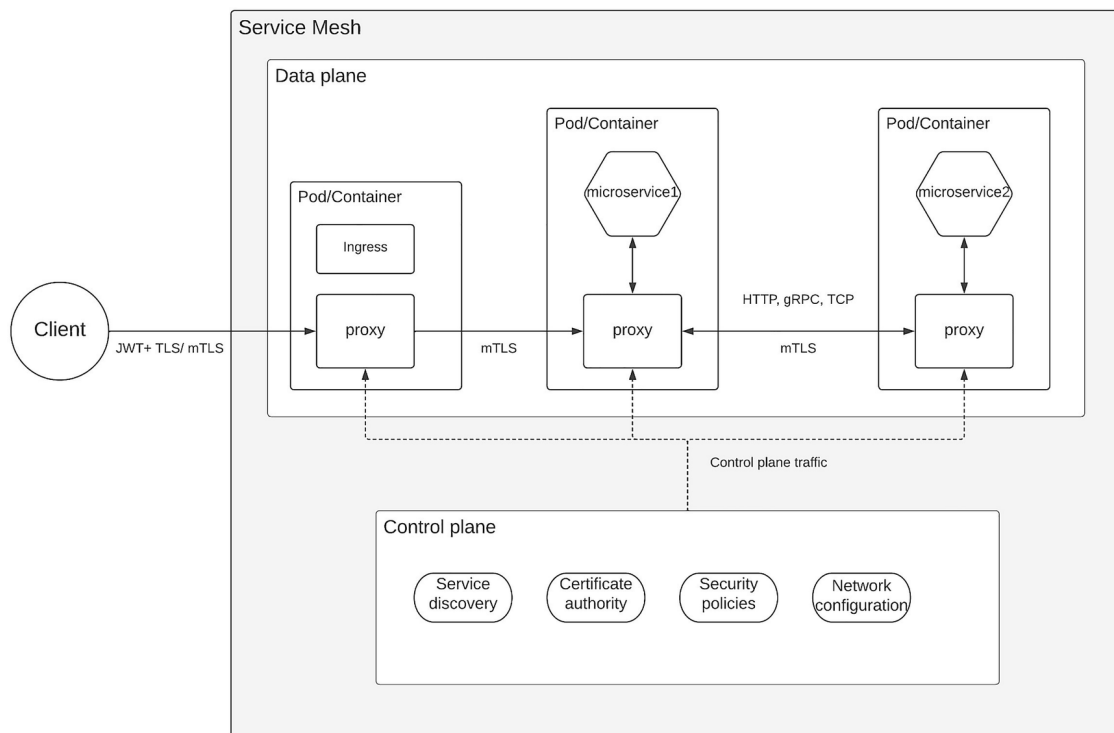
Figure 3-10 Service mesh traffic routing
