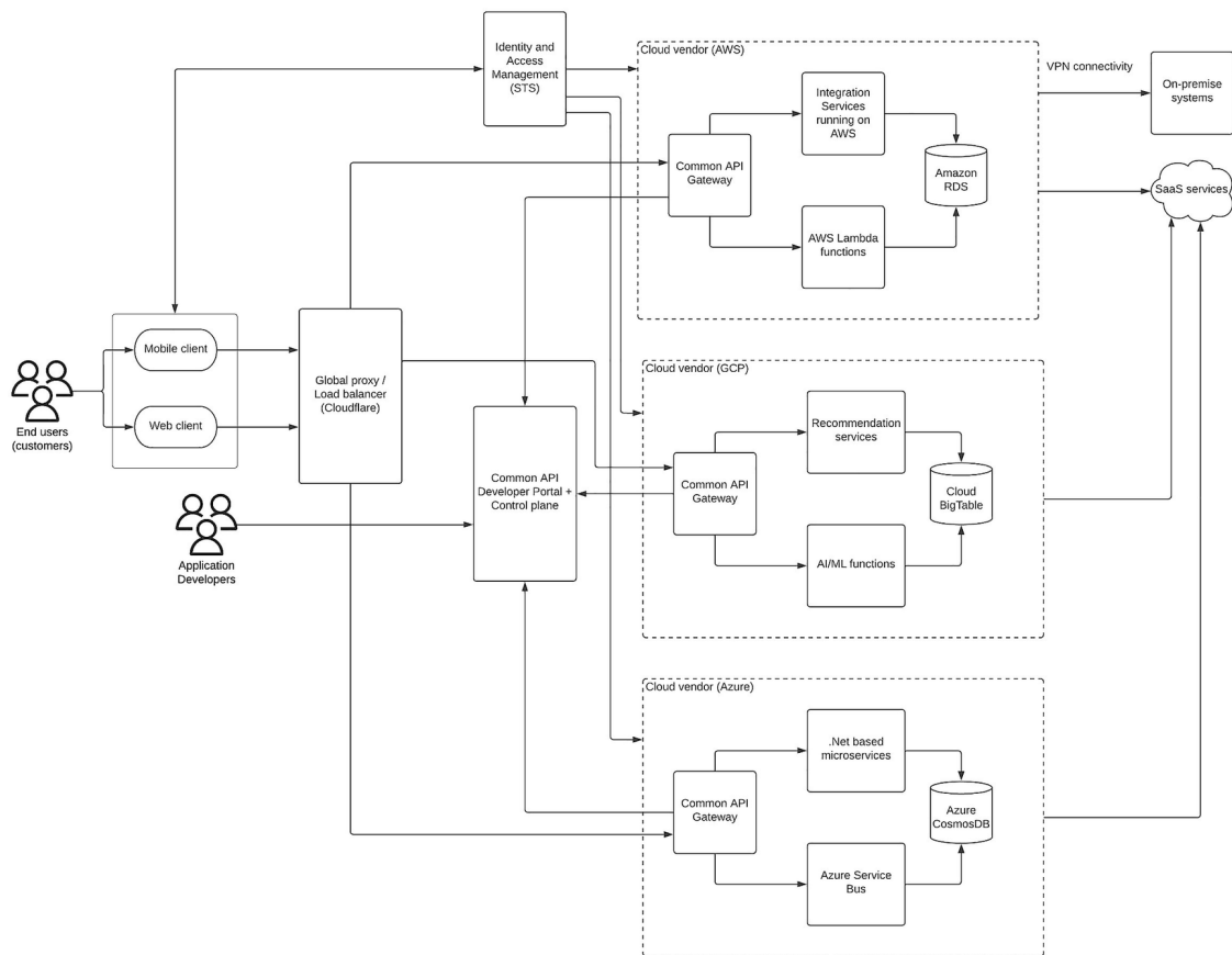
Figure 8-9 Multi-cloud deployment with a common API gateway
