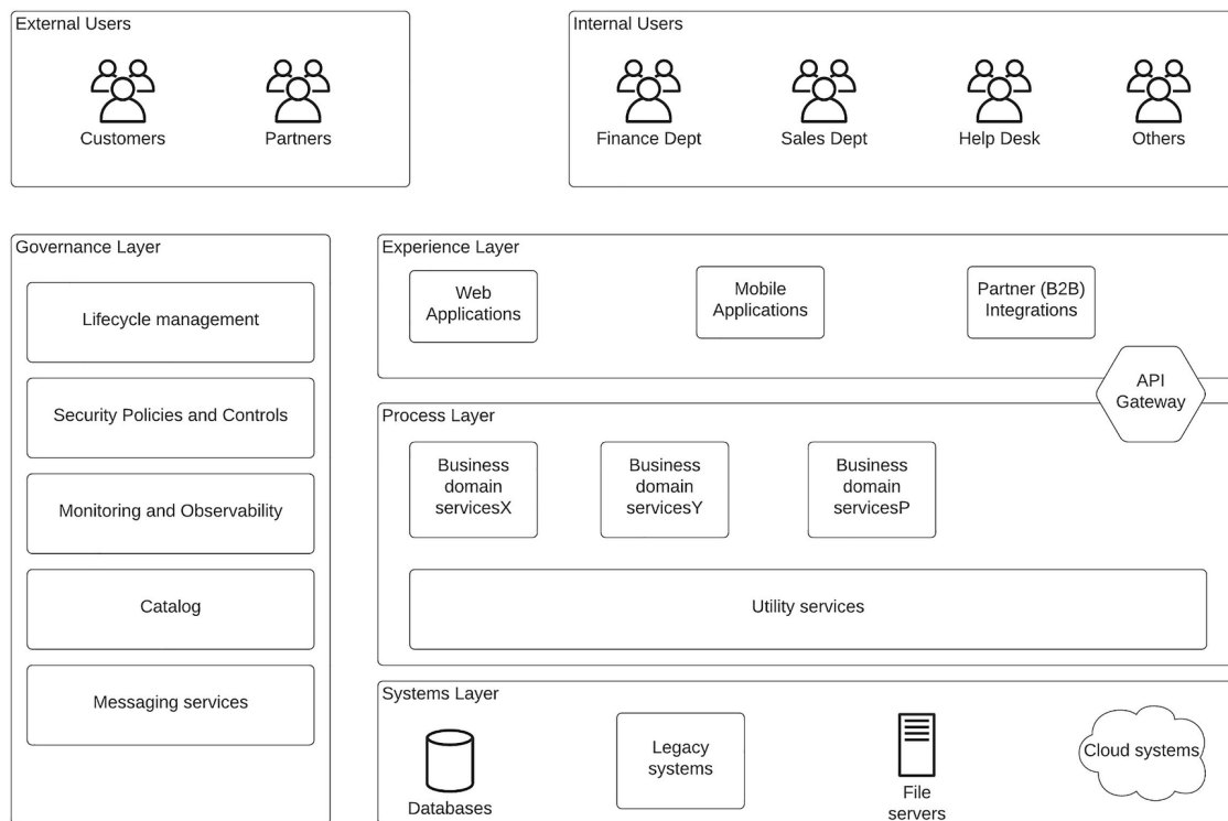
Figure 2-1 Layered enterprise architecture pattern
