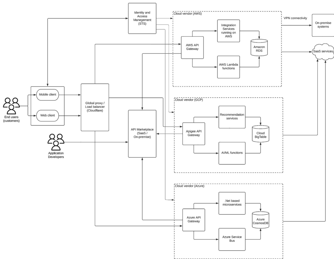
Figure 8-8 Multi-cloud deployment pattern with vendor-specific API gateways
