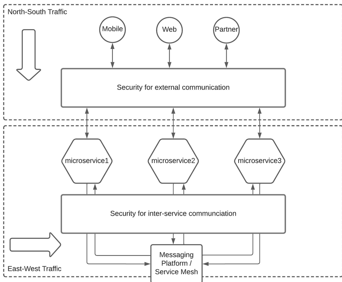
Figure 3-12 Implementing security for microservice architecture
