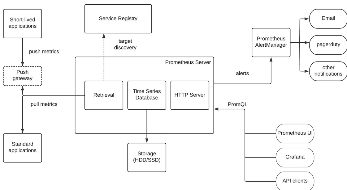
Figure 7-8 Prometheus component architecture
