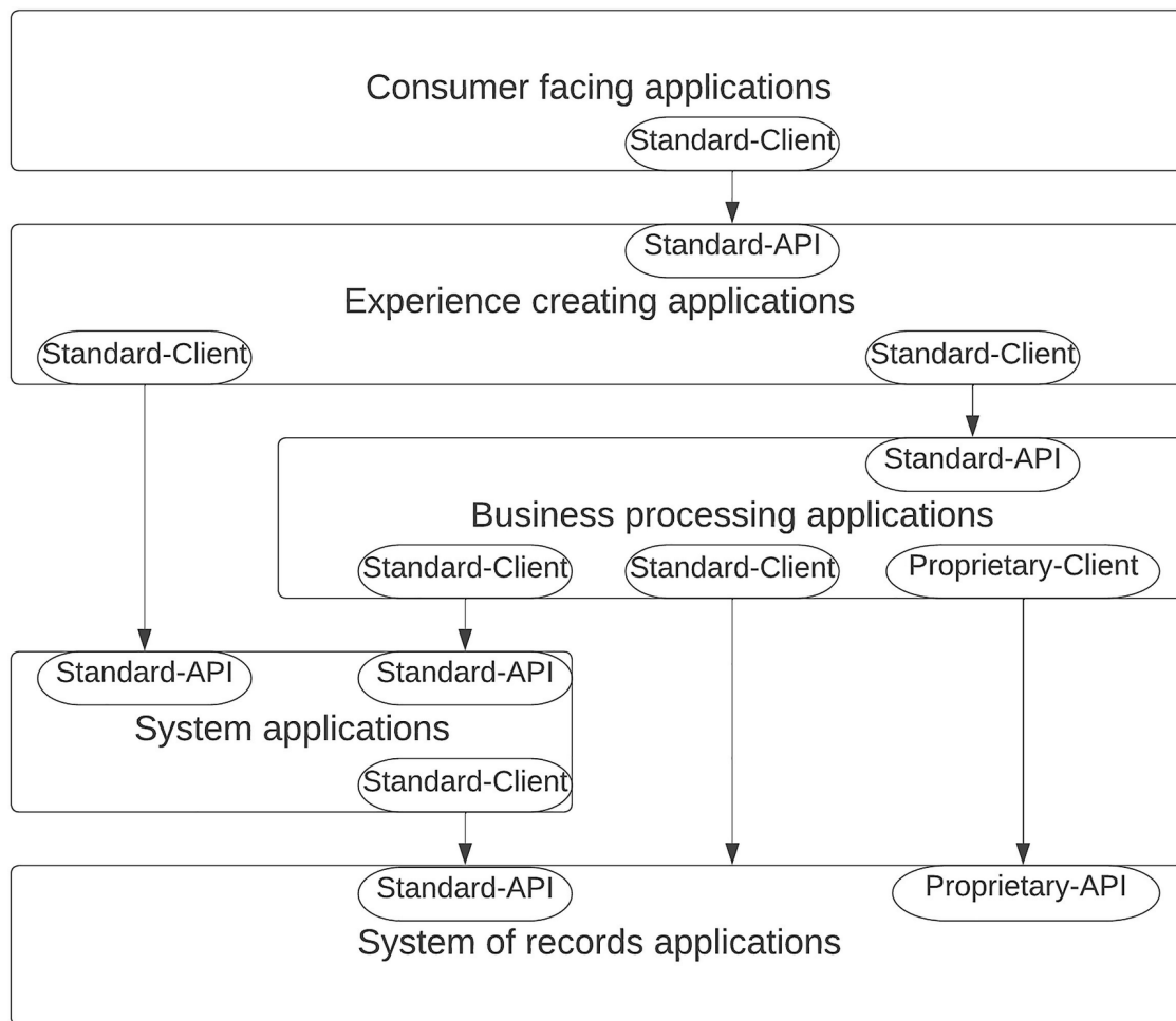
Figure 4-8 Layered architecture with API-led interoperability
