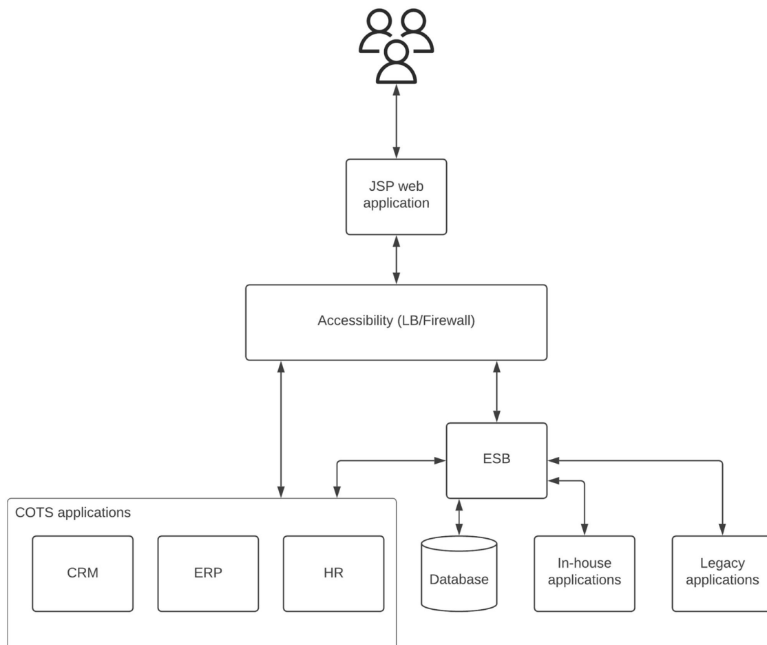
Figure 8-11 Brown-field, on-premise enterprise platform example
