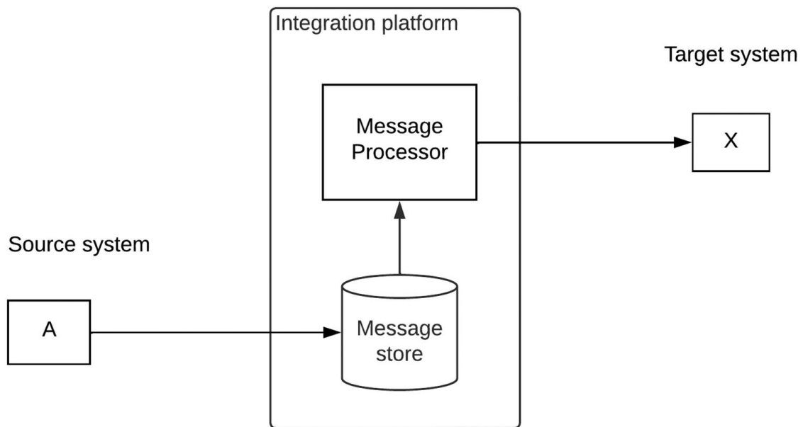
Figure 5-3 Message store and forward pattern
