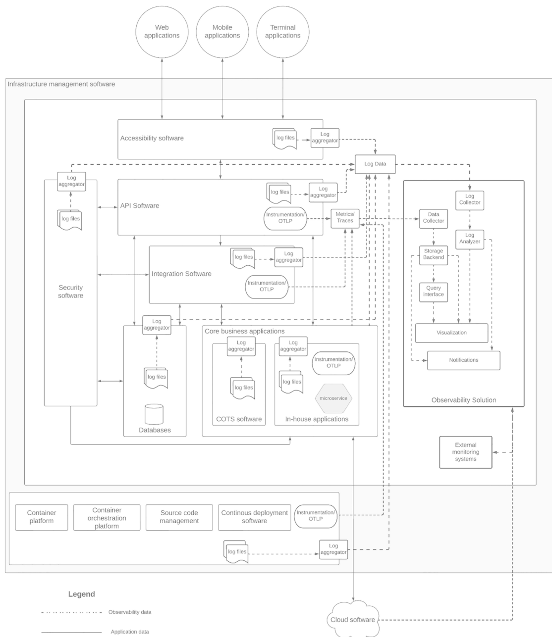
Figure 7-10 Observability solution reference architecture
