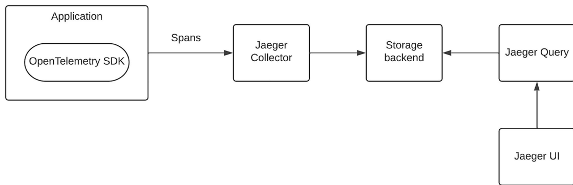
Figure 7-7 Observability with a Jaeger example
