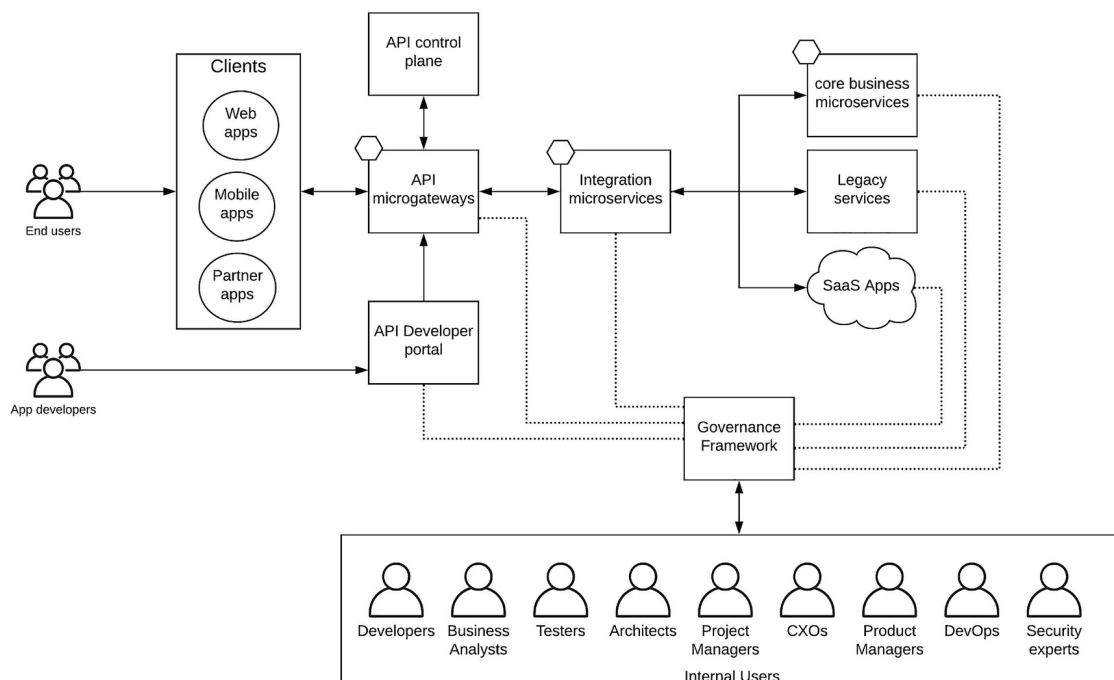
Figure 3-15 Implementing microservice governance
