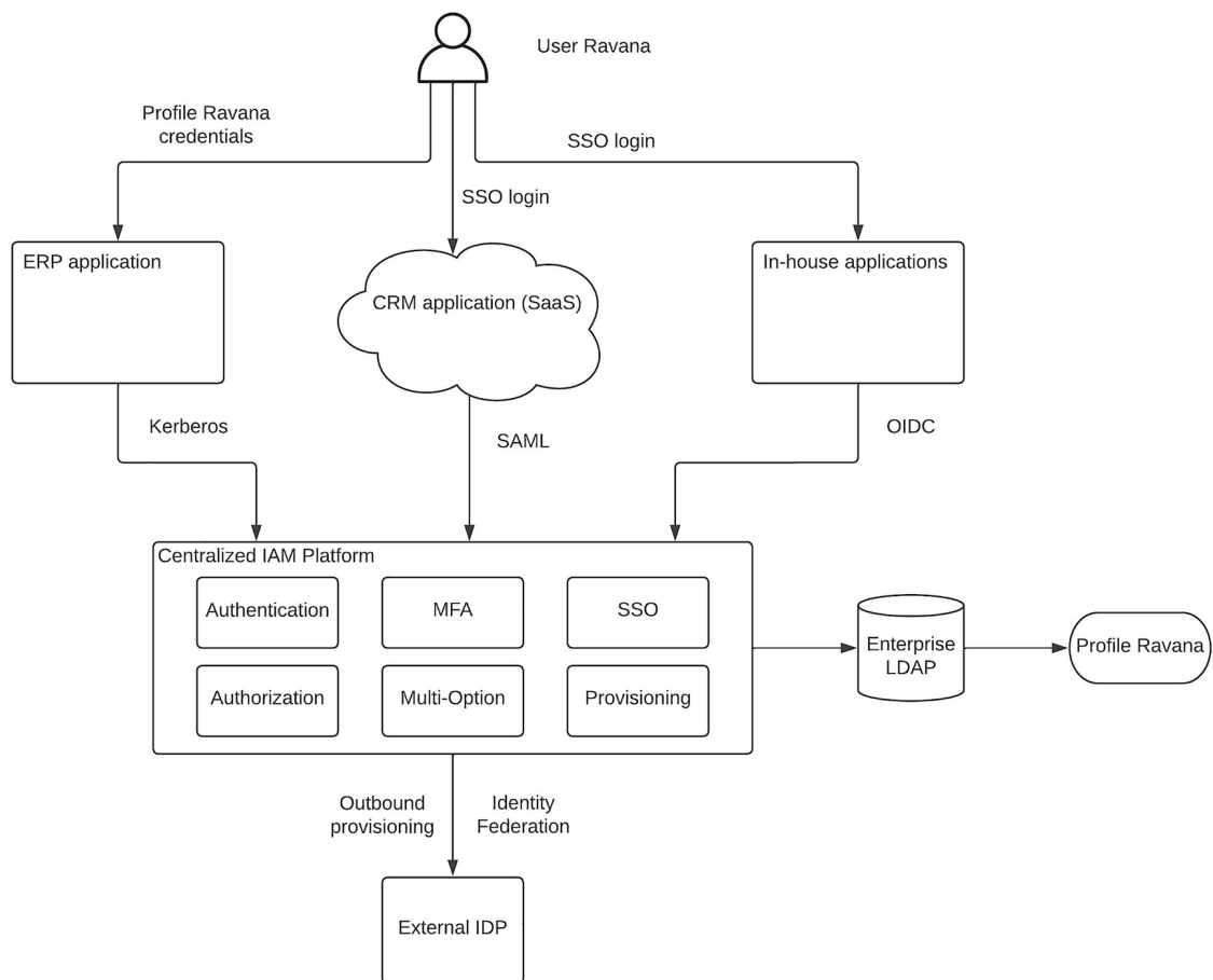
Figure 6-11 Centralized IAM pattern for enterprise security
