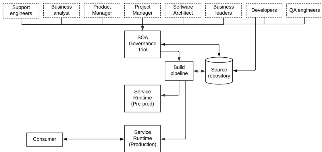
Figure 4-10 Service governance in an enterprise software system
