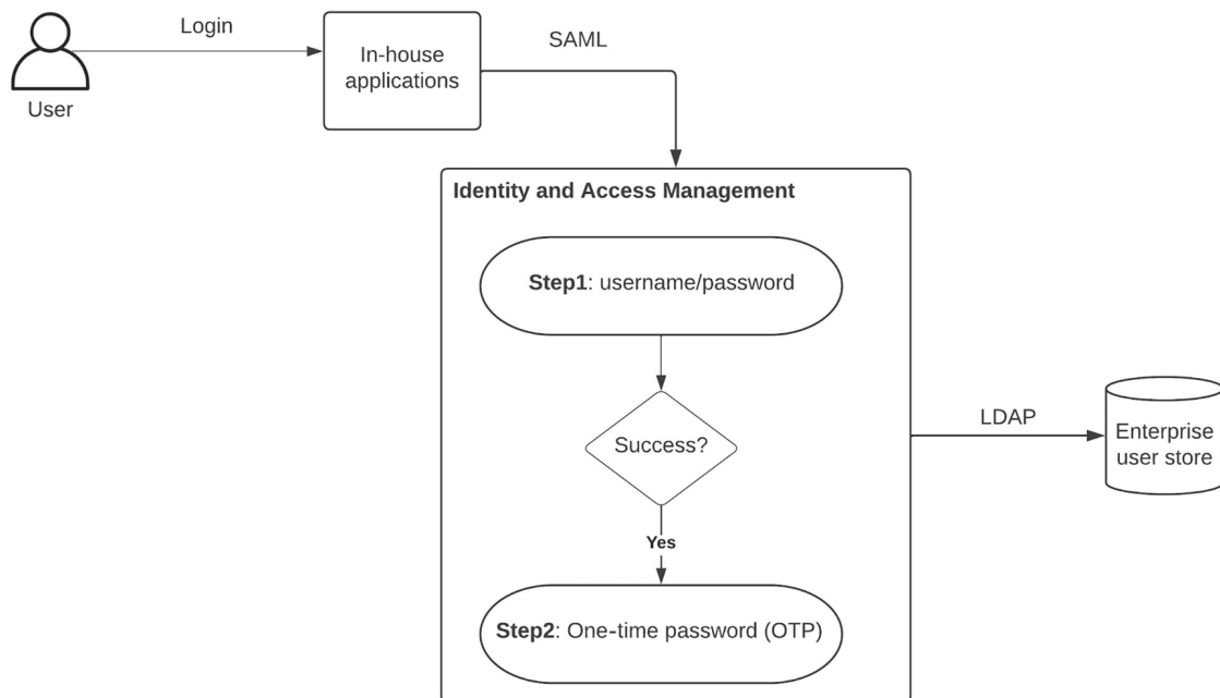
Figure 6-5 Strong authentication for enterprise security
