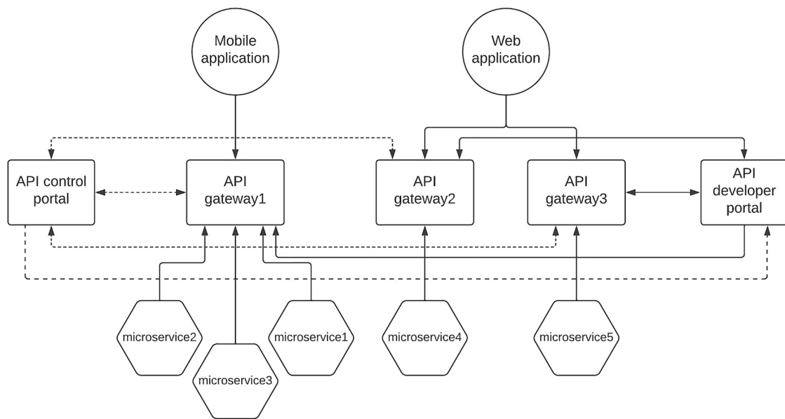
Figure 3-6 Migrating API management software to microservice architecture
