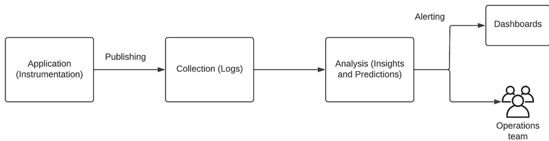
Figure 7-1 Implementing observability – functional components
