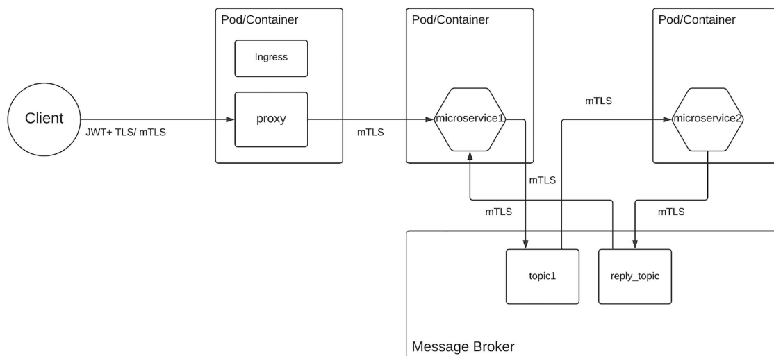
Figure 3-11 Interservice communication in MSA with the message broker
