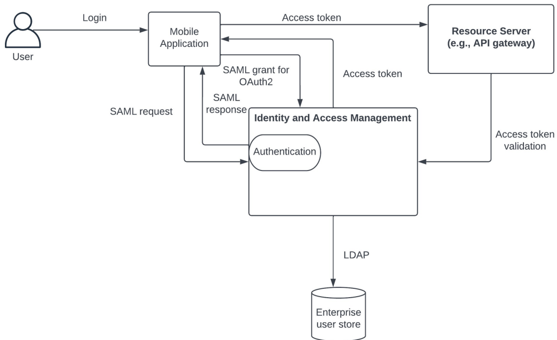
Figure 6-8 Delegated access control for enterprise security
