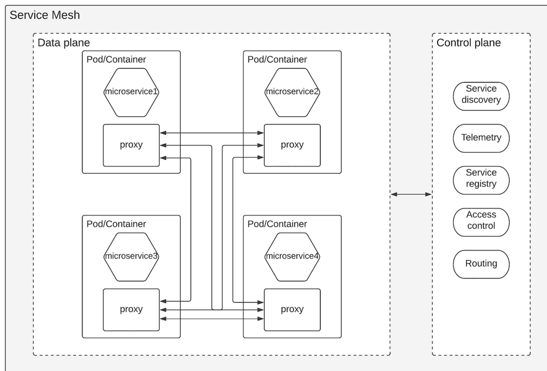
Figure 3-9 Service mesh architecture
