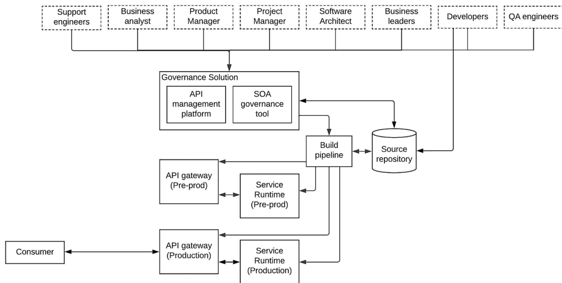
Figure 4-11 Service and API governance in an enterprise software system
