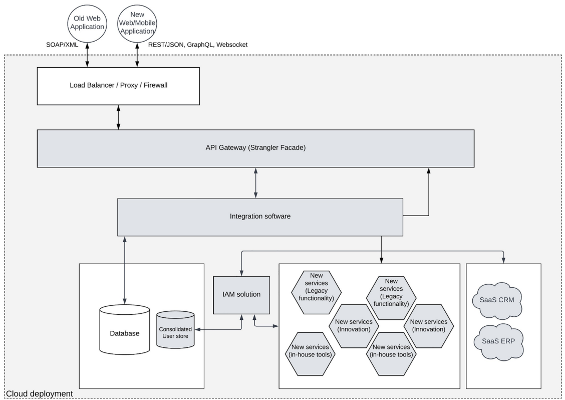
Figure 4-16 Legacy platform modernization with cloud deployment
