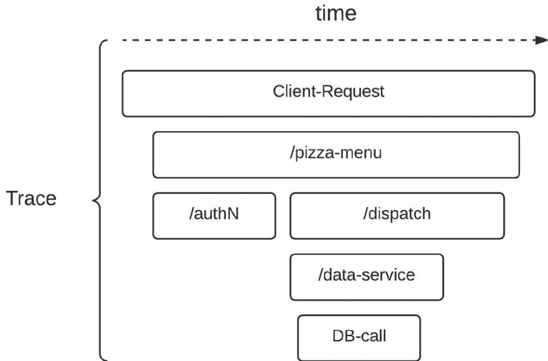
Figure 7-6 A trace in a distributed application
