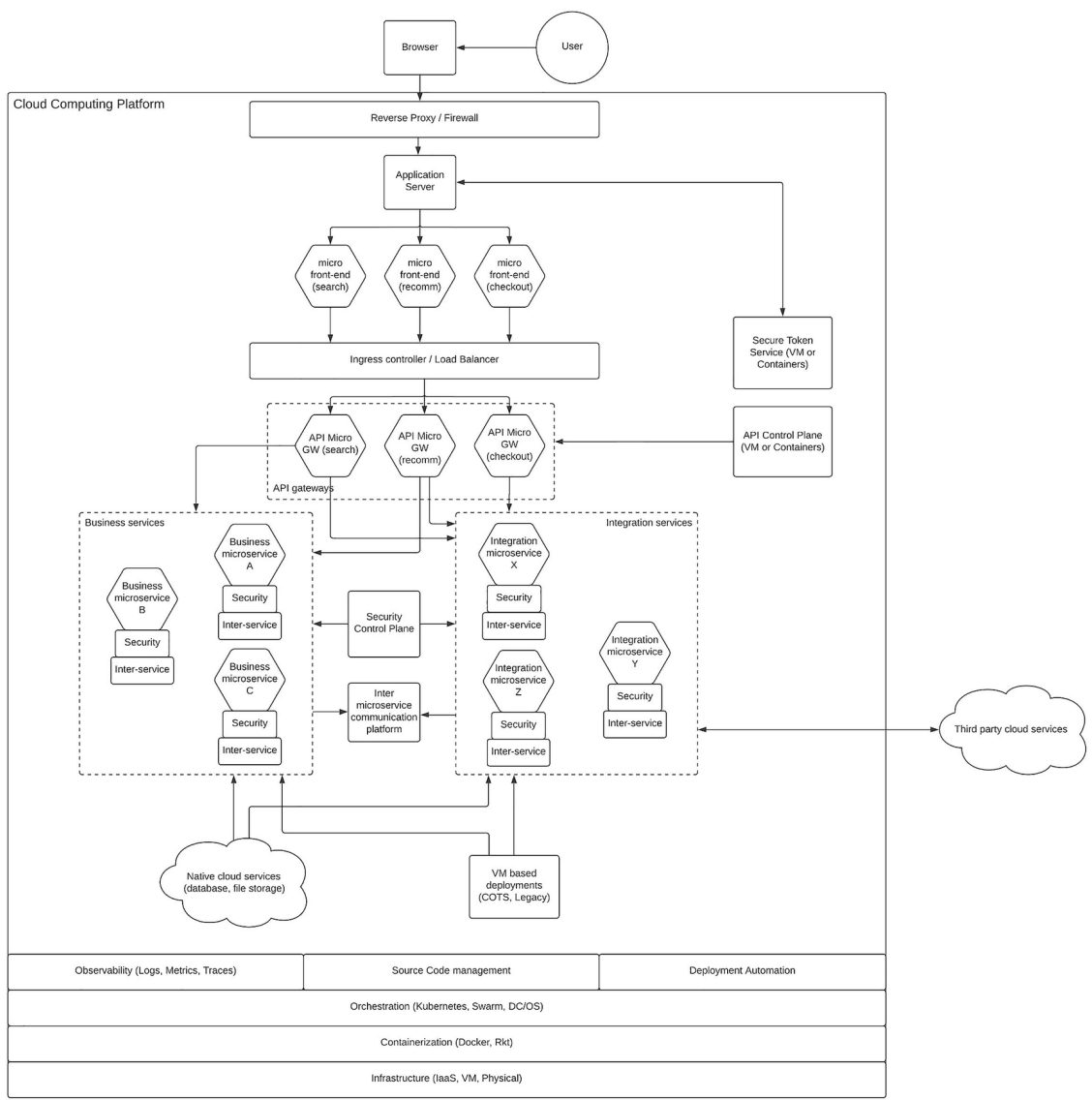
Figure 8-5 Micro-architecture pattern for an enterprise
