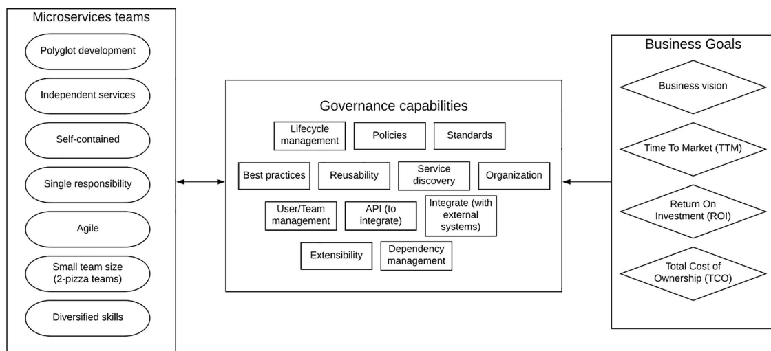
Figure 3-14 Governance capabilities of enterprise IT systems
