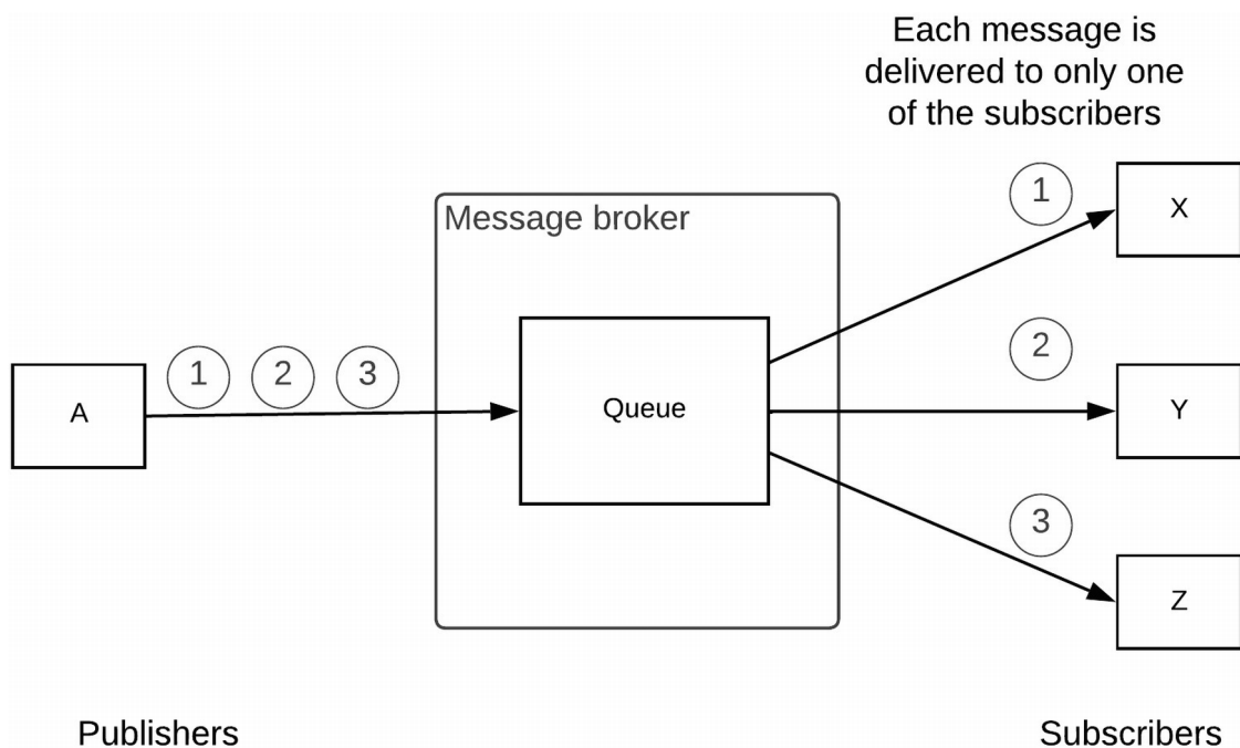
Figure 5-2 Queue-based publish-subscribe pattern
