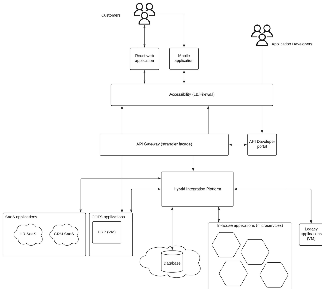
Figure 8-14 Cloud migration with a strangler facade final architecture
