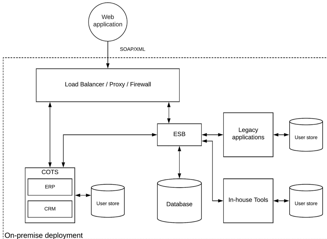
Figure 4-12 A sample legacy enterprise software system
