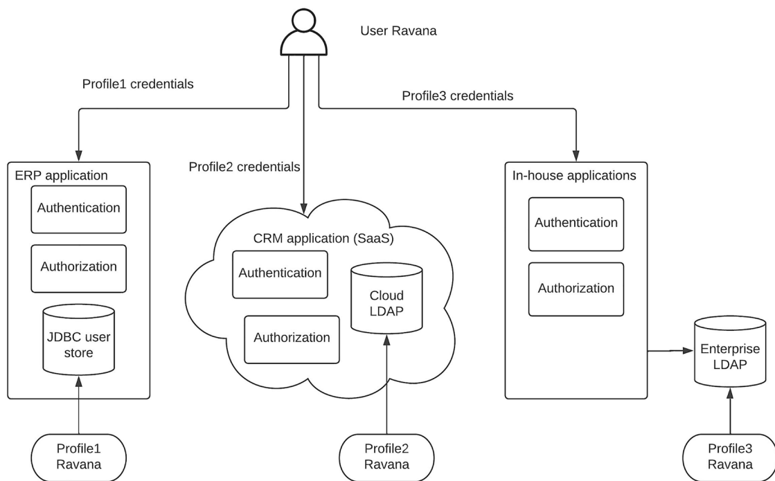
Figure 6-10 Enterprise security with application-specific security
