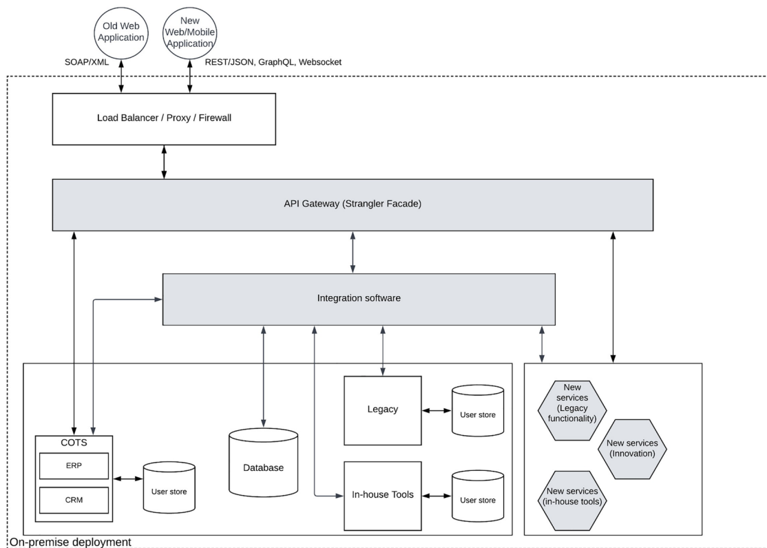
Figure 4-14 Legacy platform modernization with API gateway and integration software
