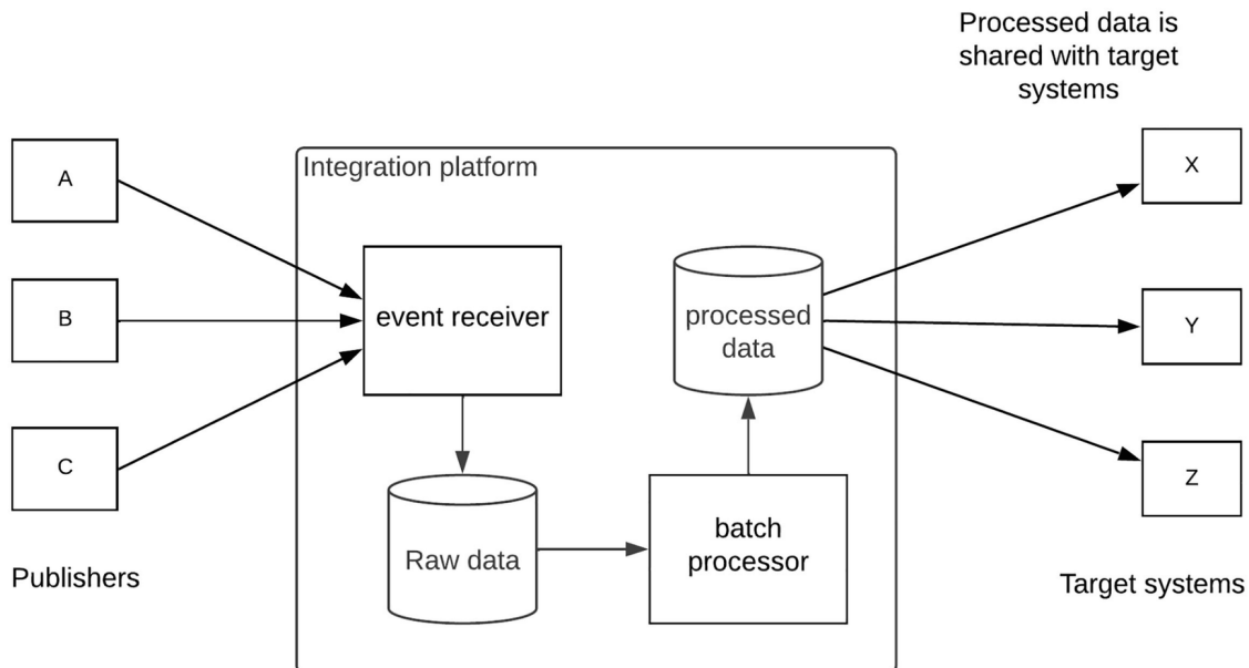
Figure 5-5 Batch processing pattern
