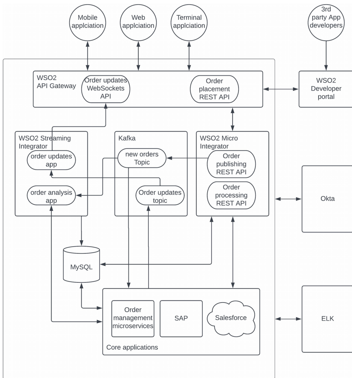
Figure 5-9 Event-driven enterprise software system with Kafka
