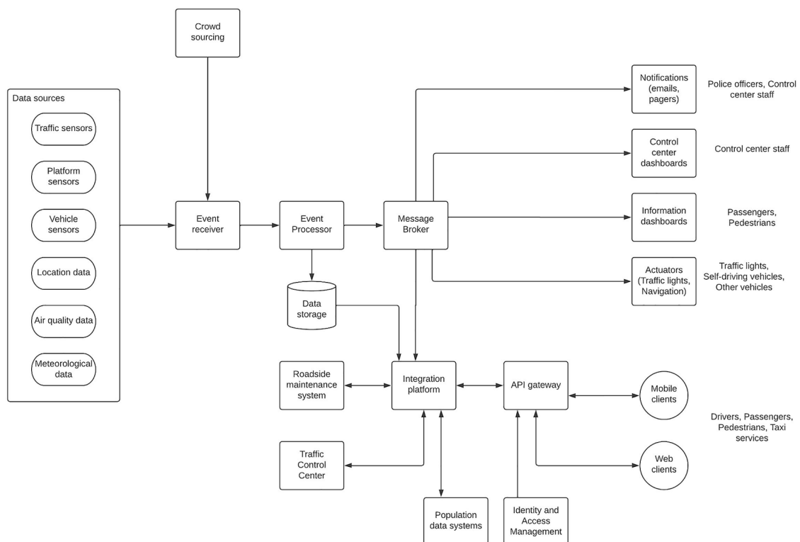
Figure 9-1 Solution architecture for ground transportation system
