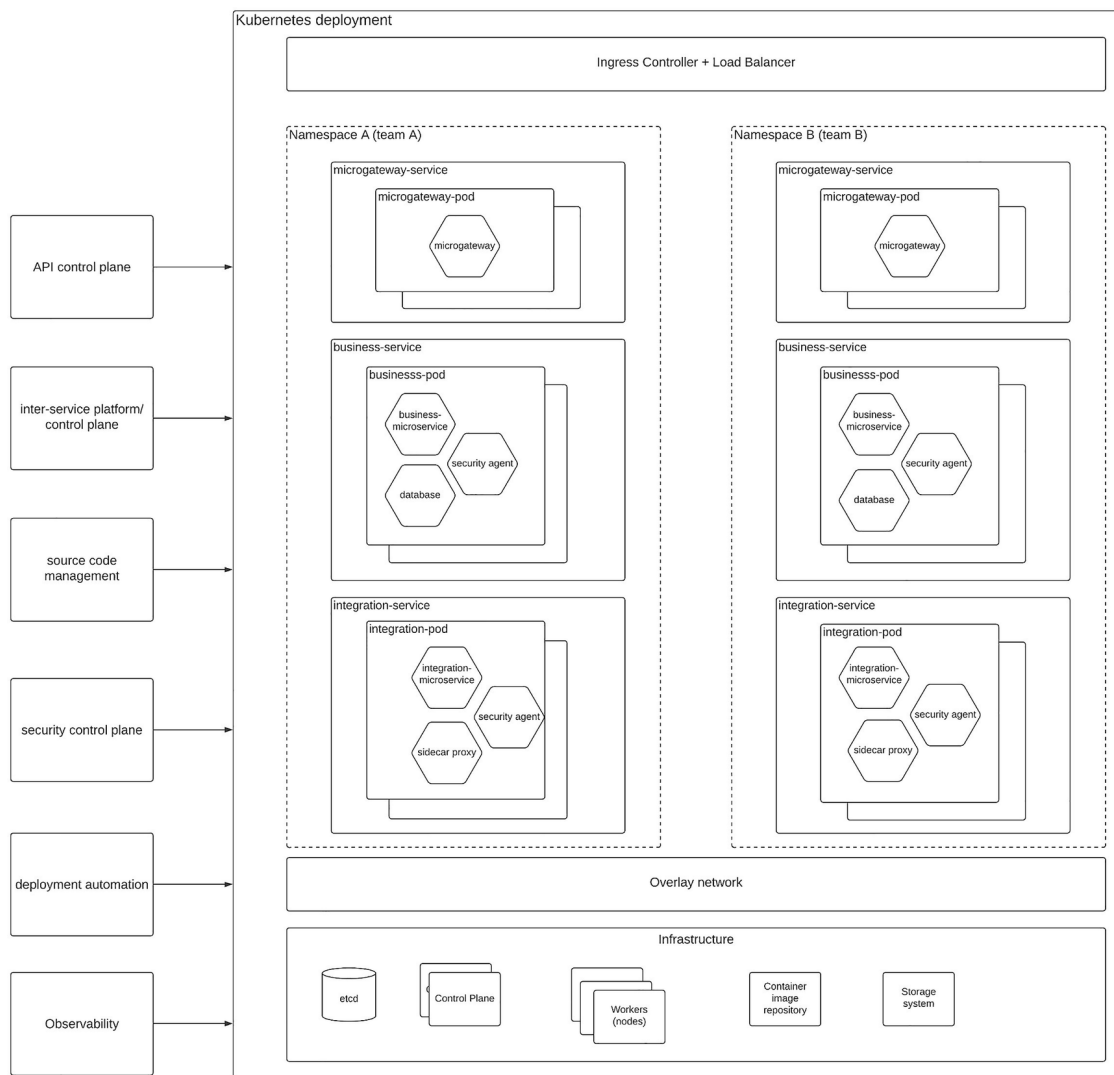
Figure 8-7 Kubernetes-based deployment pattern
