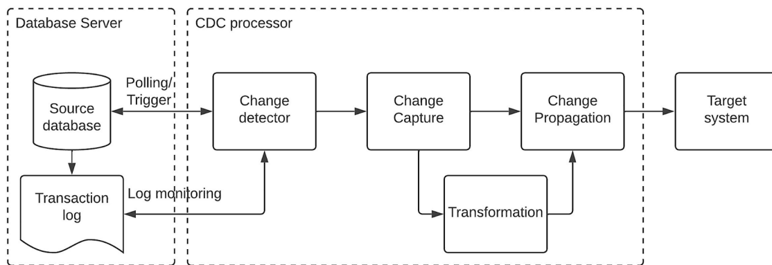
Figure 5-10 Change data capture working model
