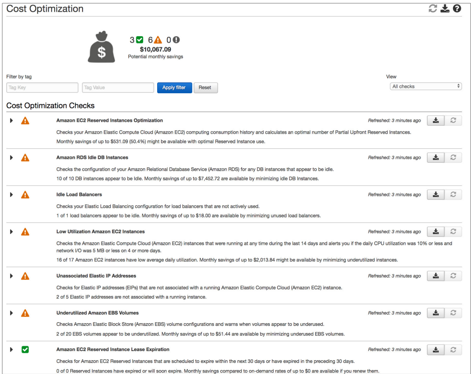
Figure 9-3 Trusted Advisor
