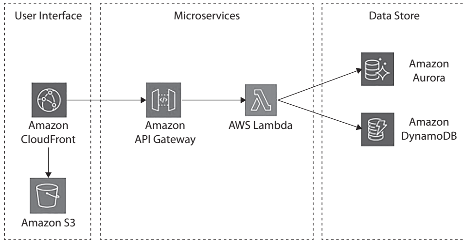
Figure 7-3 Microservices architecture with AWS Lambda
