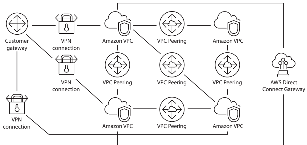
Figure 3-8 Network topology without Transit Gateway
