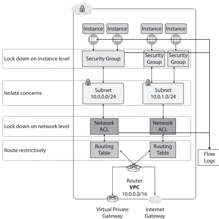
Figure 7-22 VPC Flow Logs capture
