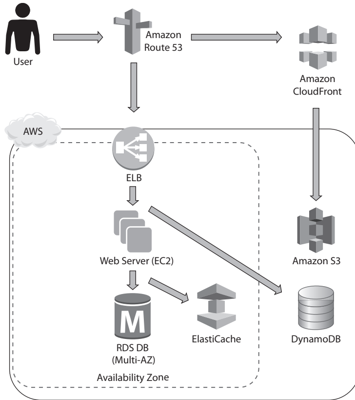
Figure 9-8 Leveraging multiple storage options
