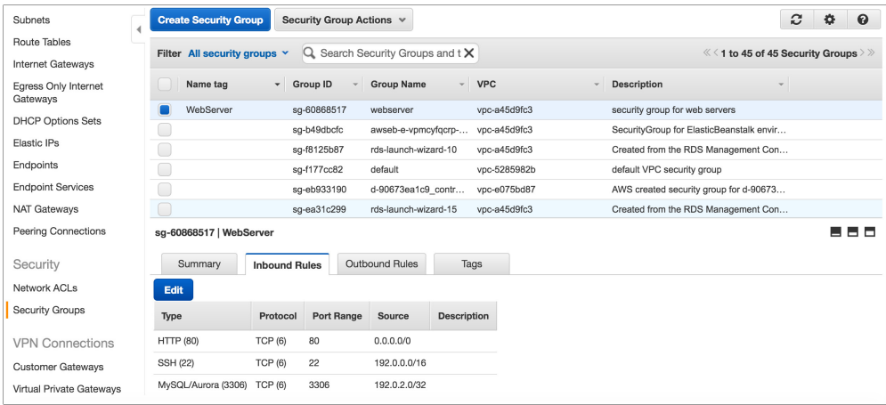
Figure 3-2 Security group
