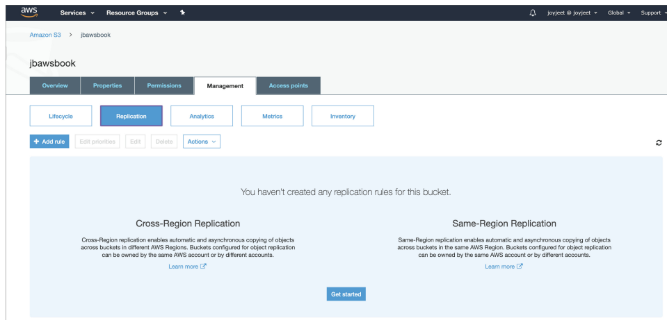
Figure 2-3 Getting started
